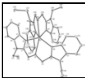
Fig. 1. Molecular structure and atom numbering for the cation. Hydrogen atoms have been omitted for clarity and the displacement ellipsoids are shown at the 30% probability level.
